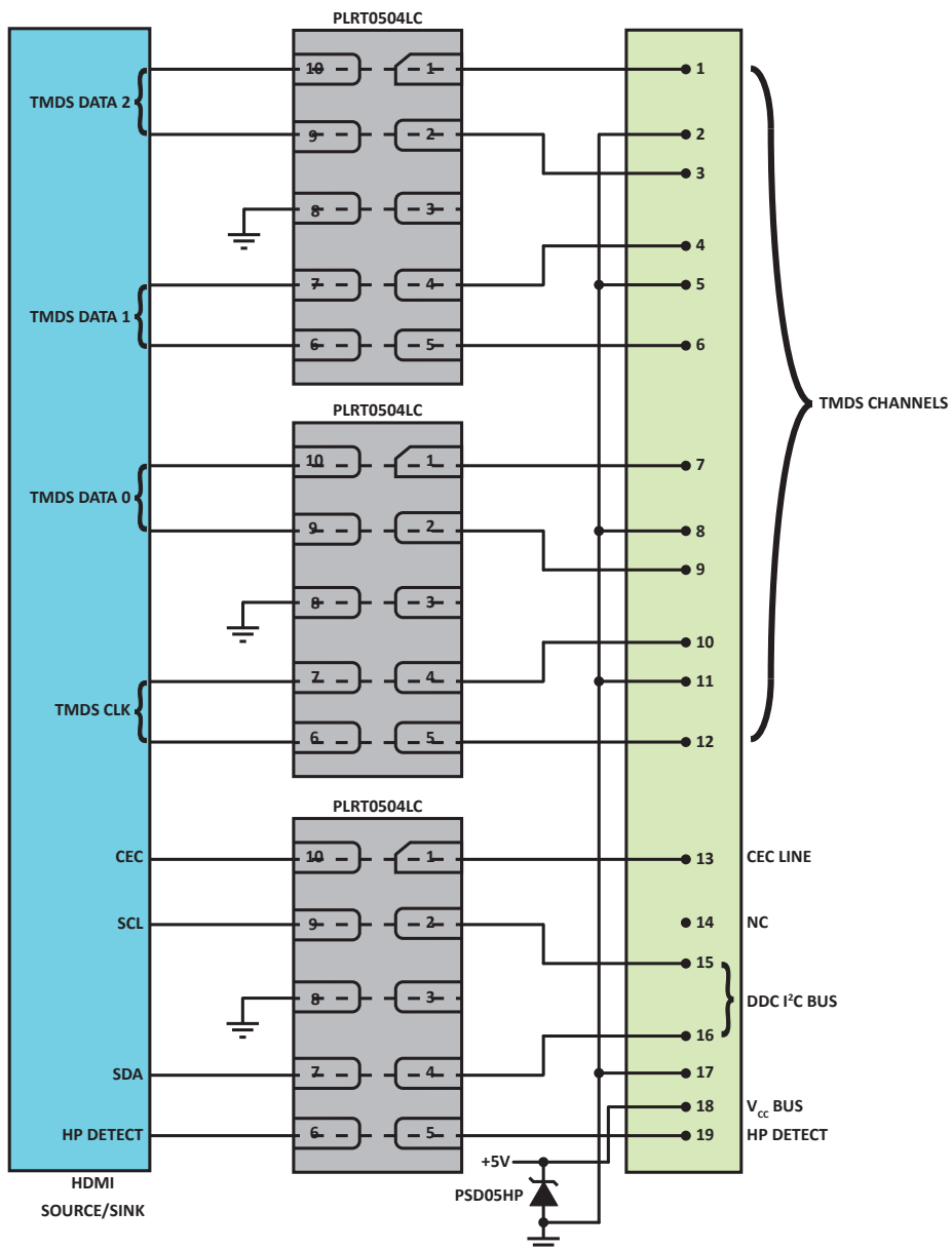
DO160 Sec. 25 ESD Protection, HDMI 2.0 Interface Protection Using the PLRT0504LC and PSD05HP for VCC Bus Protection
