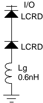
FIGURE 1 SPICE MODEL FOR PLC497
