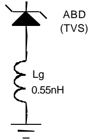
FIGURE 1 SPICE MODEL FOR PSD SERIES
