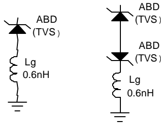
FIGURE 1 SPICE MODEL FOR PSOT & PSOTxxC SERIES
