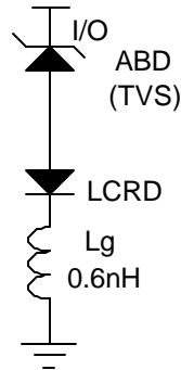
FIGURE 1 SPICE MODEL FOR PSOTxxLC SERIES
