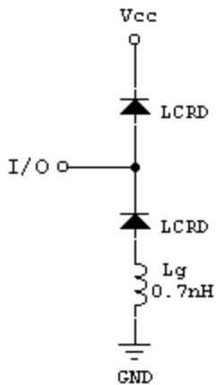
FIGURE 1 SPICE MODEL FOR PSRDA70-4
