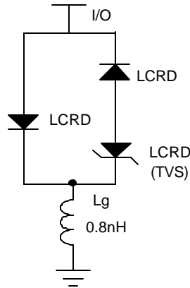
FIGURE 1 SPICE MODEL FOR SM16LC SERIES
