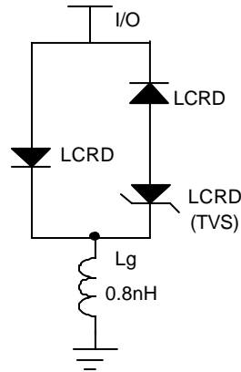
FIGURE 1 SPICE MODEL FOR USB04 SERIES
